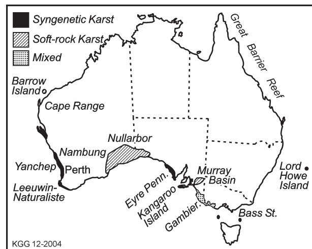
Figure 19: Areas of syngenetic and soft-rock Karst in Australia.
