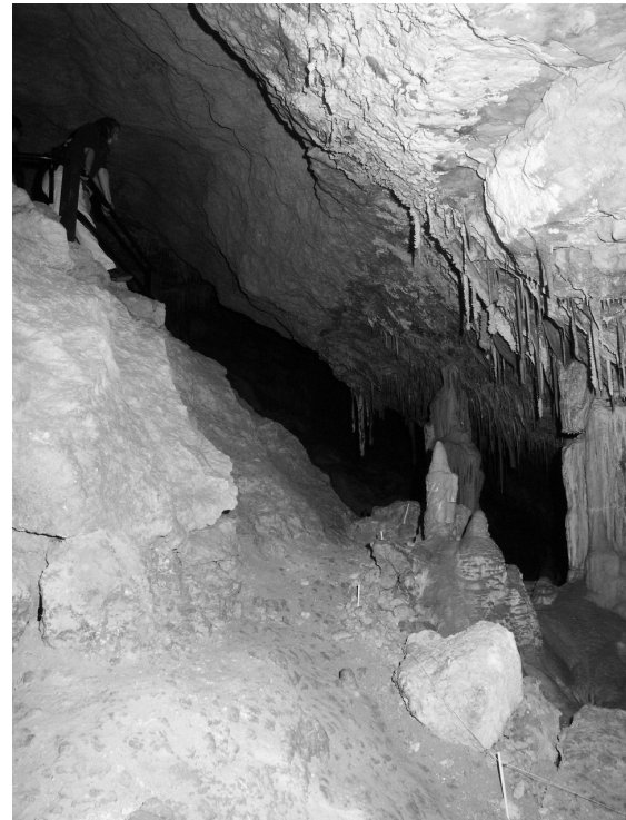
Figure 18: An "Inclined fissure" left at the side of a rubble mound in a collapse dome. Grant Hall, 5U-1, Naracoorte, South Australia.
